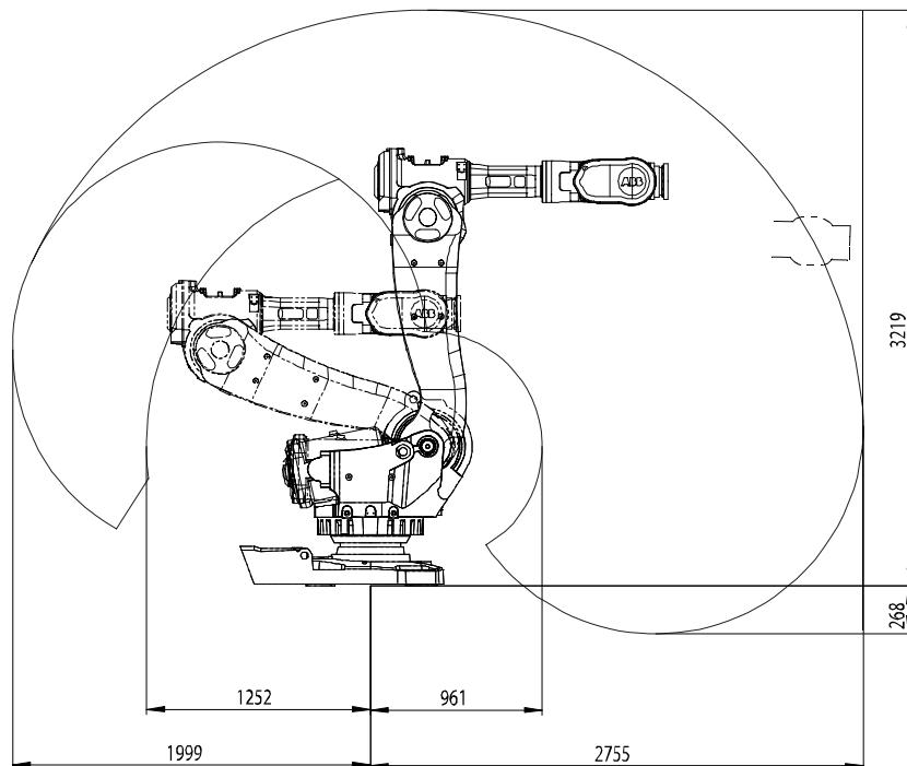
IRB 6650-200/2.75
