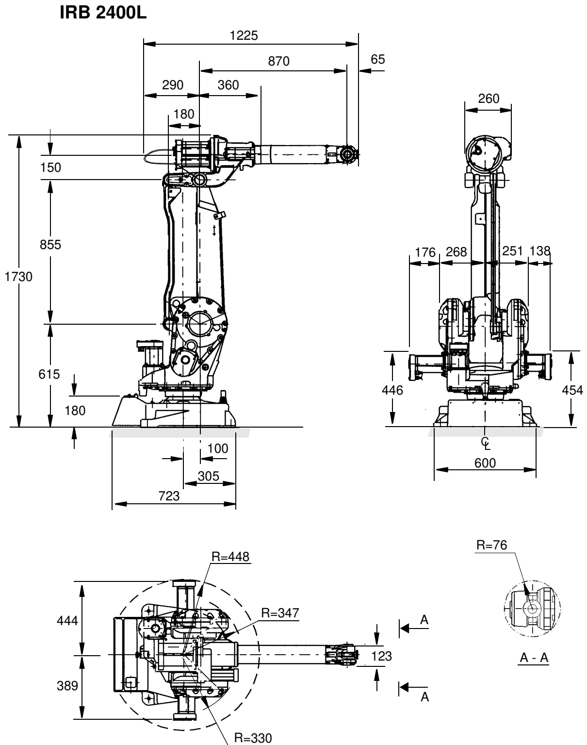
Figure 2 View of the manipulator from the side, rear and above (dimensions in mm).
