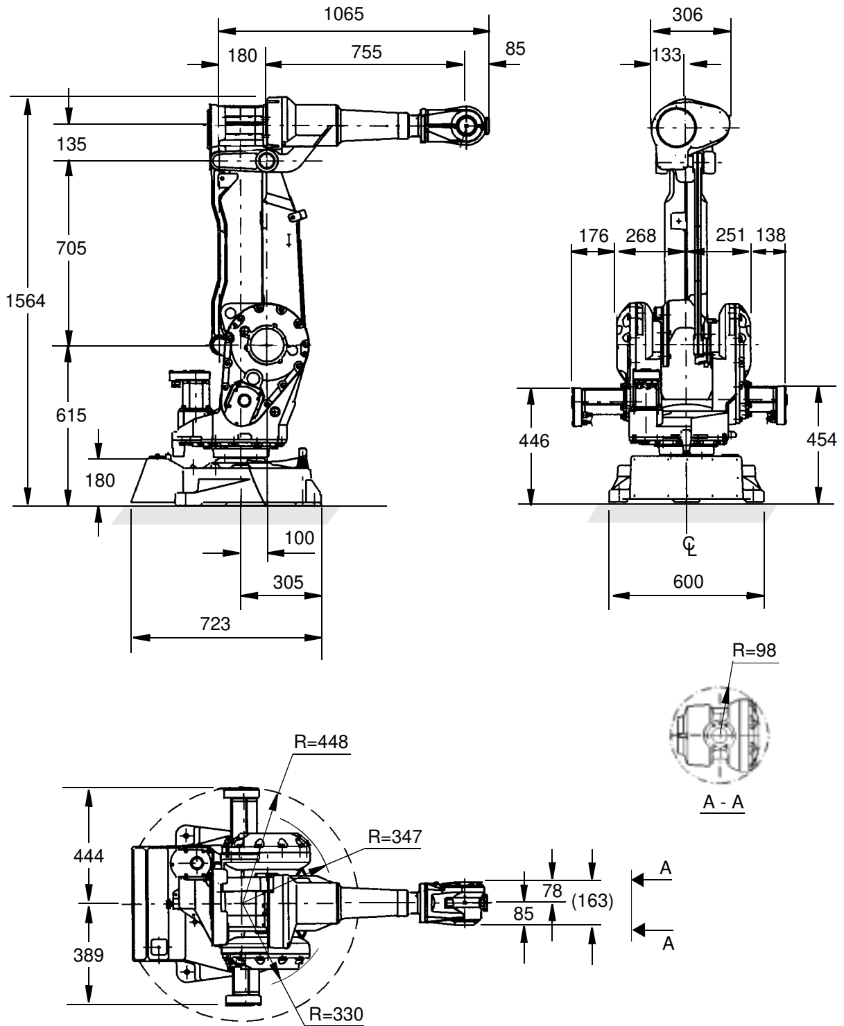
Figure 3 View of the manipulator from the side, rear and above (dimensions in mm).
