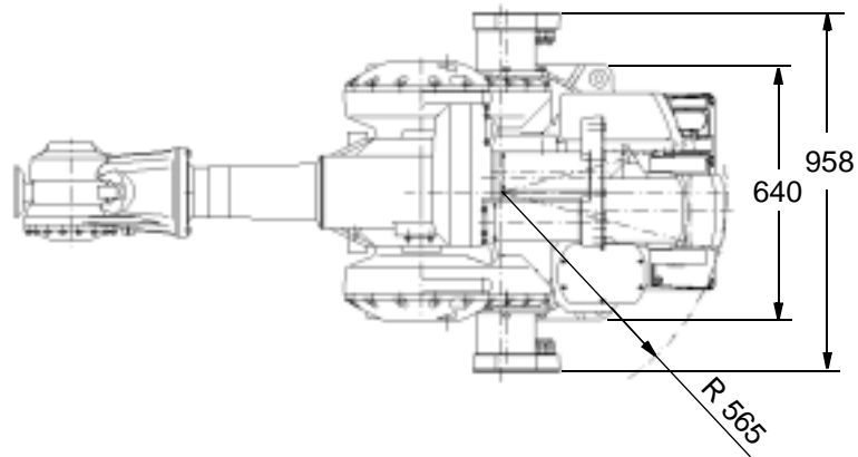
Figure 3 View of the manipulator from above (dimensions in mm).
