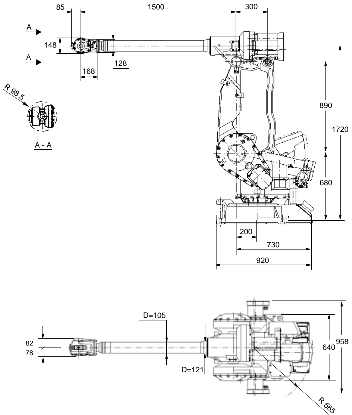
Figure 4 View of the manipulator from the side and above (dimensions in mm).
