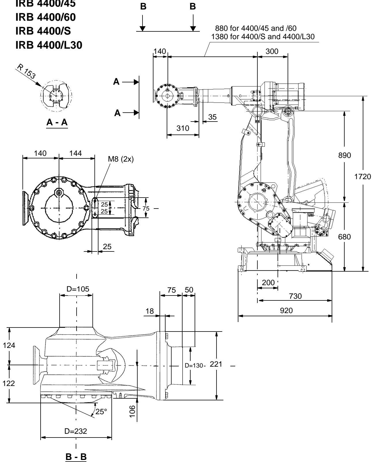
Figure 2 View of the manipulator from the side (dimensions in mm).
